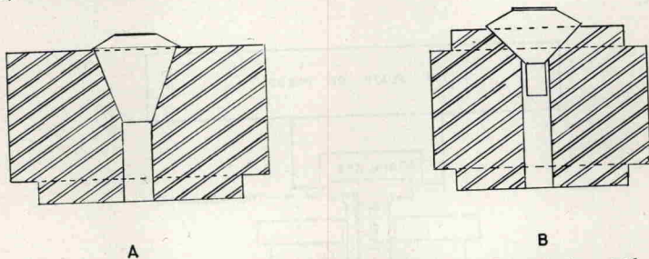
Fig. 2. Pistons and holders: A. 20° cone, used only for cemented carbides. B. 45° cone in configuration used for high speed and stellite pistons. When using this cone angle for carbides, the upper and lower cylindrical sections are omitted, and the acute angle between the two cones is flush with the top of the holder. In both cases, .003" copper sheet was placed between the pistons and holders to serve as lubricant.
